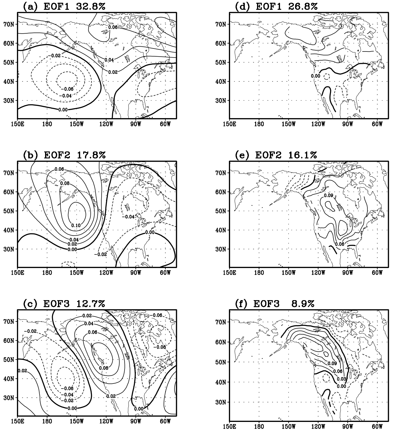
Figure 3: The first 3 EOFs of the winter 500-mb geopotential height (Z500) anomalies (left column) and surface air temperature (SAT) anomalies (right column). Solid curves denote positive contours, dashed curves, negative contours, and thick curves, zero contours. The contour interval is 0.02 in panels (a), (b) and (c), and 0.03 in panels (d), (e) and (f). The EOFs have been normalized to unit norm. If the sign in panel (b) is reversed, then over the North American continent, the patterns in the left column generally agree with those in the right column.
