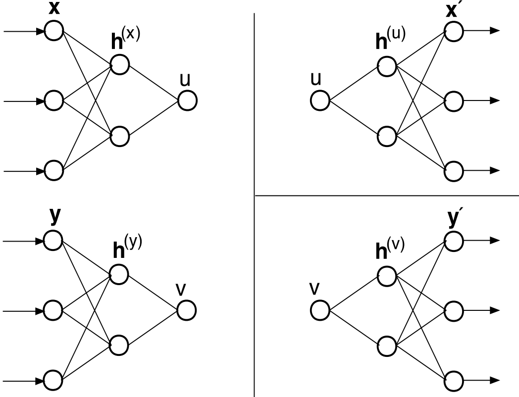
Figure 2: A schematic diagram illustrating the three feed-forward NNs used to perform nonlinear canonical correlation analysis (NLCCA). In the applications here, all the hidden layers \mathbf{h}^{(x)} , \mathbf{h}^{(y)} , \mathbf{h}^{(u)} and \mathbf{h}^{(v)} have 3 neurons each.
