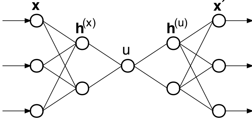
Figure 1: A schematic diagram of the neural network (NN) model for calculating nonlinear PCA (NLPCA). The network is a standard feed-forward NN (i.e. multi-layer perceptron), consisting of several layers of ‘neurons’ (i.e. variables). The network maps from the input layer on the left to the encoding layer, then to the bottleneck layer (with a single neuron), to the decoding layer, then finally to the output layer on the right. In the applications here, the hidden layers \mathbf{h}^{(x)} and \mathbf{h}^{(u)} both have 3 neurons, while the input \mathbf{x} are the 5 leading principal components.
